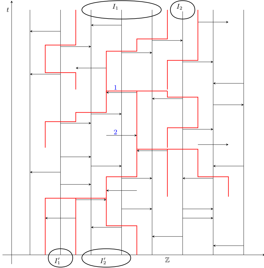
FIG 5. Superduality: If \eta_t \cap I_1 \neq \emptyset and \eta_t \cap I_2 \neq \emptyset , then there must exist a backward 3-path as drawn such that \eta_0 \cap I'_1 \neq \emptyset and \eta_0 \cap I'_2 \neq \emptyset . Between times when the 3-path renews itself, it consists of three dual coalescing random walk paths which form the boundaries of two adjacent intervals as in Figure 4. Cooperative branching arrows such as the one marked “1” may be used to renew the 3-path by splitting one of its paths into three new paths, but they do not need to be used such as the cooperative branching arrow 2.
