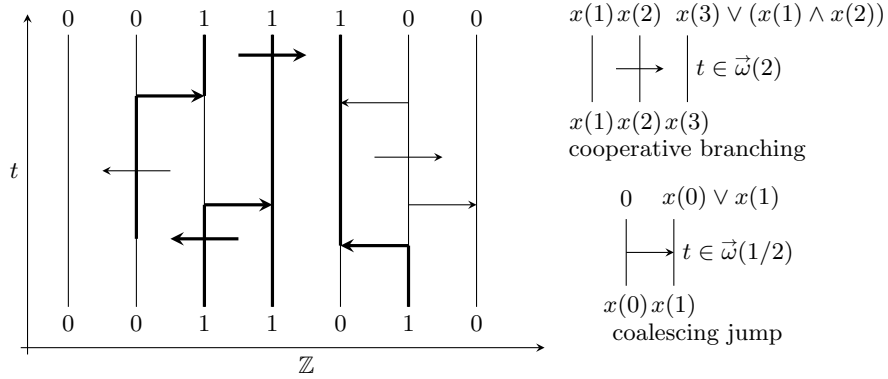
FIG 1. Example of a graphical representation with explanation of the rules. Bold lines indicate the presence of a particle. Arrows that are used by a particle to jump through, or by a pair of particles to give birth to a third particle are also drawn bold, regardless of whether such a particle lands on an occupied site or not.
