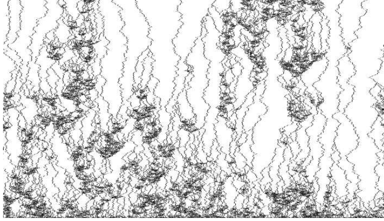
FIG 3. Simulation of a near-critical cooperative branching-coalescent with \lambda = 7/3 on a lattice of 700 sites with periodic boundary conditions, started from the fully occupied initial state. Space is plotted horizontally, time vertically, and black indicates the presence of a particle.
