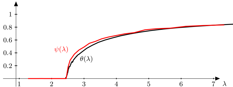
FIG 2. Density \theta(\lambda) of the upper invariant law and survival probability \psi(\lambda) (plotted in black and red, respectively) of the cooperative branching-coalescent as a function of the cooperative branching rate.
