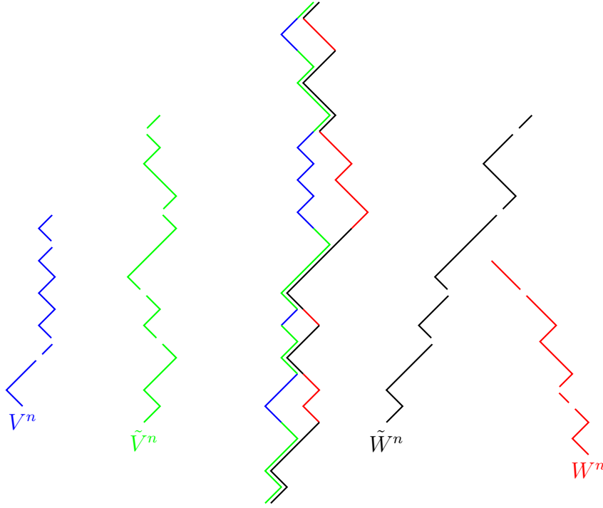
Figure 5.6: Decomposition of a left path and a right path (middle picture) into four random walks V^{(n)}, \tilde{V}^{(n)}, \tilde{W}^{(n)} and W^{(n)} . Here V^{(n)} and \tilde{V}^{(n)} have a drift to the left while \tilde{W}^{(n)} and W^{(n)} have a drift to the right. The random walks \tilde{V}^{(n)} and \tilde{W}^{(n)} are highly correlated, but V^{(n)} and W^{(n)} are independent of each other and of the pair (\tilde{V}^{(n)}, \tilde{W}^{(n)}) .
