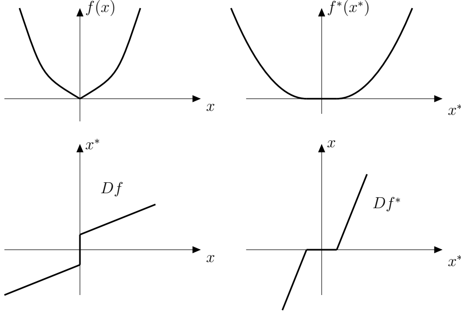
Figure 2.2: Legendre transform of a non-smooth function.
