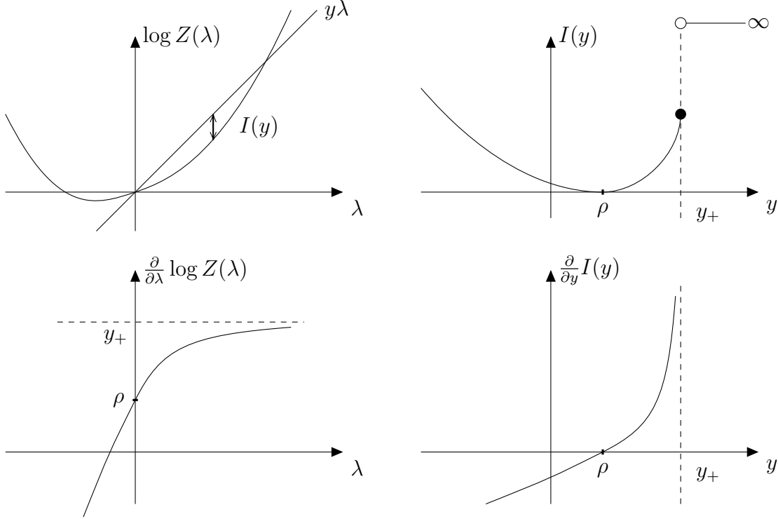
Figure 2.4: Definition of the rate function in Cramér's theorem. The functions below are derivatives of the functions above, and inverses of each other.
