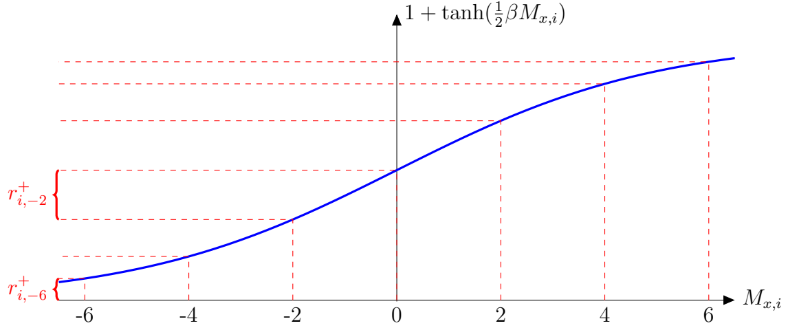
Figure 4.2: Definition of the rates r_{i,L}^+ from (4.31). In this example N = 6 and \beta = 0.4 .
