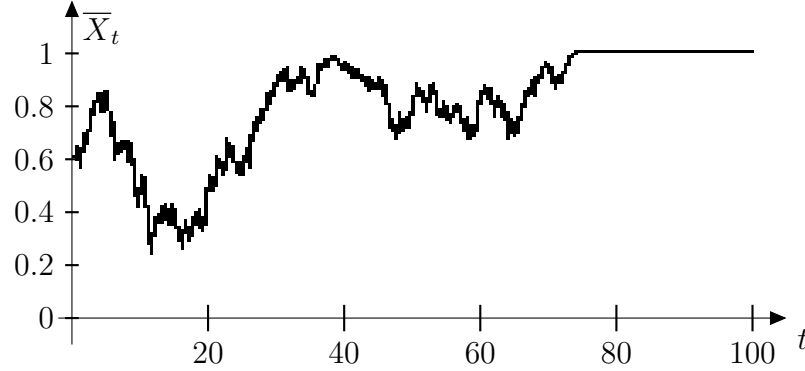
Figure 3.6: The fraction of type 1 individuals in the mean-field voter model from (3.25) on N = 100 sites. This process approximates the Wright-Fisher diffusion.
