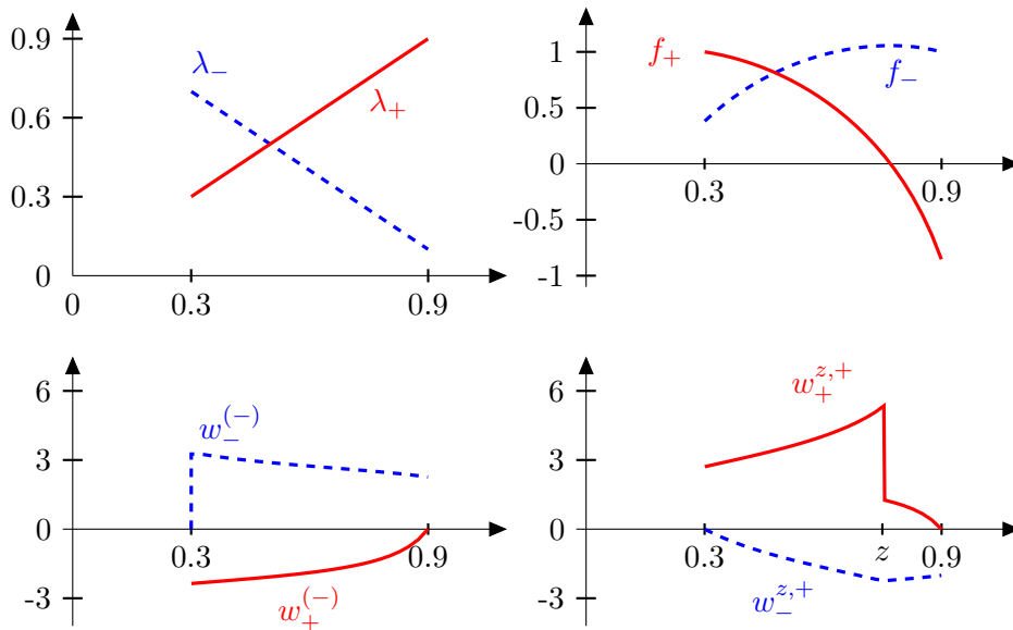
Figure 3: The solution (f_-, f_+) to Luckock's equation, as well as two examples of weight functions (w_-, w_+) as in Theorem 9. In this example, I = (0.3, 0.9) , \lambda_-(x) = 1 - x , and \lambda_+(x) = x . The lower left picture shows the weight functions w_{\pm}^{(-)} = w_{\pm}^{I,-} while the lower right picture shows the weight functions w_{\pm}^{z,+} for z = 0.75 .
