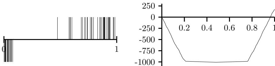
Figure 1: Simulation of the “uniform” Stigler-Luckock model with I = (0, 1) , \lambda_-(x) = 1 - x , and \lambda_+(x) = x . On the left: the state X_{250} of the order book after the arrival of 250 traders, starting from the empty initial state. On the right: the distribution function x \mapsto X_k([0, x]) of the random signed measure X_k after the arrival of k = 10,000 traders.
