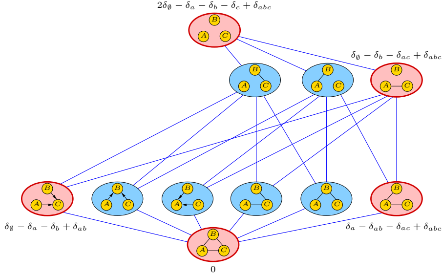
Fig. 1. The essential graphs and (some) standard imsets in the case of three variables.
